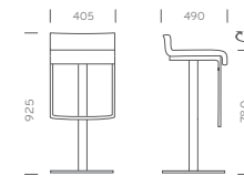
Colonna Column 50x50 | 400x400
